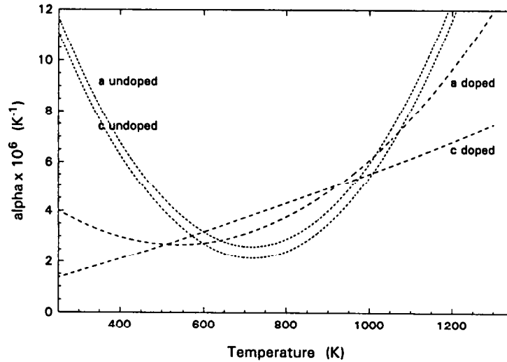
Fig. 4. The temperature dependence of the coefficient of thermal expansion \alpha_T of doped and undoped sodium \beta'' -alumina was determined from the fits to the unit cell parameters shown in Fig. 3.
