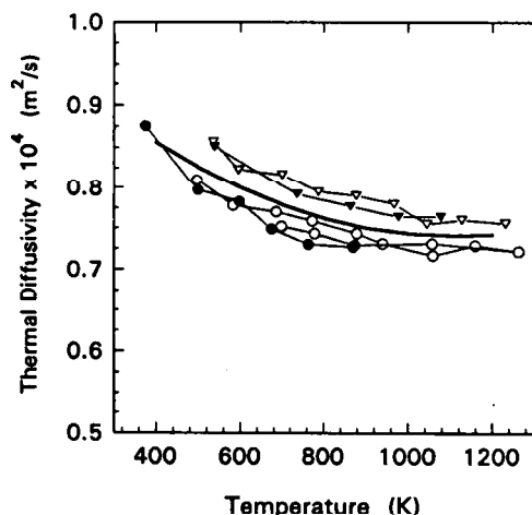
Fig. 1. The thermal diffusivity of \beta'' -alumina polycrystalline ceramic was measured using a flash method. Circles are sample 1, triangles are sample 2. The heavy line is the smoothed value of thermal diffusivity.
