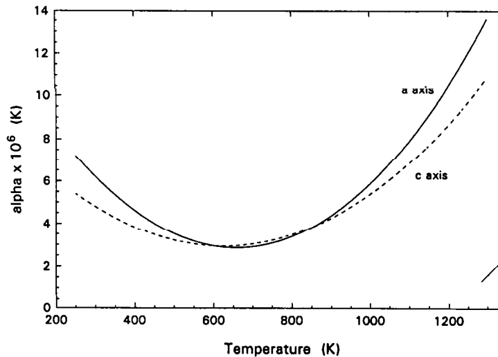
Fig. 5. The temperature dependence of the coefficient of thermal expansion was determined from the combined doped and undoped \beta'' -alumina ceramic unit cell parameters.
